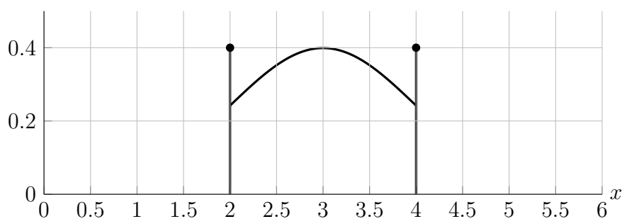
Censored data from below and above
