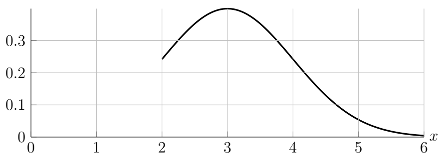
Censored data from above
